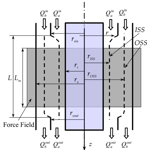
Fig. 1. Schematic diagram of an annular quadrupole magnetic flow sorter.
