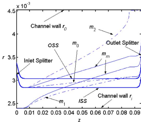
Fig. 4. Particle trajectories and ISS, OSS stream-lines in the separation channel, where the total flow Q = 60 ml/min, the magnet flux density B_0 = 1.334 T. The magnetophoretic mobilities are: m_0 = 3.98 \times 10^{-4} , m_1 = 8.09 \times 10^{-4} , m_2 = 21.38 \times 10^{-4} , and m_m = 12.0 \times 10^{-4} mm 3 /TAs, respectively.
