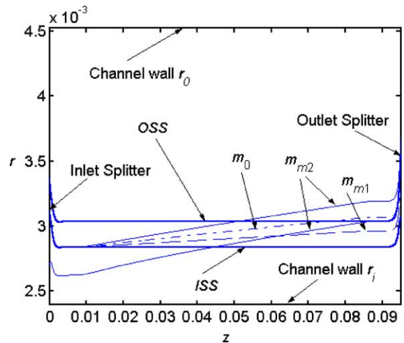
Fig. 6. Particle trajectories and ISS, OSS stream-lines in the separation channel, where the total flow Q = 10 ml/min, the magnet flux density B_0 = 0.775 T. The magnetophoretic mobilities are: m_0 = 1.91 \times 10^{-4} , m_1 = 3.91 \times 10^{-4} , m_2 = 10.58 \times 10^{-4} , m_{m1} = 1.0 \times 10^{-4} , and m_{m2} = 3.0 \times 10^{-4} mm 3 /TAs, respectively.
