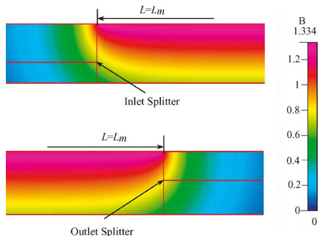
Fig. 8. The fringing force field at the splitters, B_0 = 1.334 T. Here, variation of the fringing field around the circumference of the annular channel is ignored.
