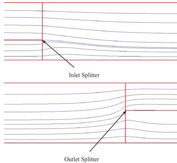
Fig. 2. Streamlines at the separation channel inlet and outlet, Q = 60 ml/min.
