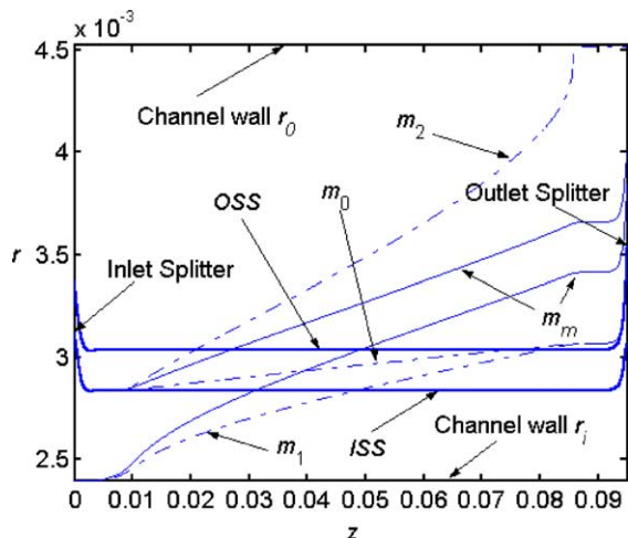
Fig. 5. Particle trajectories and ISS, OSS stream-lines in the separation channel, where the total flow Q = 10 ml/min, the magnet flux density B_0 = 0.775 T. The magnetophoretic mobilities are: m_0 = 1.91 \times 10^{-4} , m_1 = 3.91 \times 10^{-4} , m_2 = 10.58 \times 10^{-4} , and m_m = 7.0 \times 10^{-4} mm 3 /TAs, respectively.
