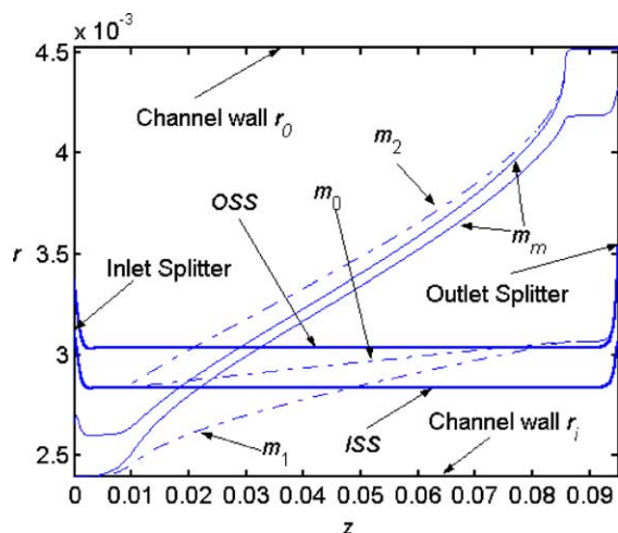
Fig. 7. Particle trajectories and ISS, OSS stream-lines in the separation channel, where the total flow Q = 10 ml/min, the magnet flux density B_0 = 0.775 T. The magnetophoretic mobilities are: m_0 = 1.91 \times 10^{-4} , m_1 = 3.91 \times 10^{-4} , m_2 = 10.58 \times 10^{-4} , and m_m = 12.0 \times 10^{-4} mm 3 /TAs, respectively.
