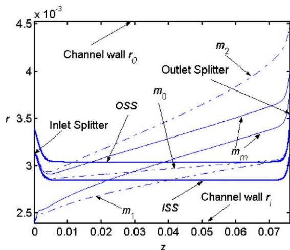
Fig. 9. Particle trajectories and ISS, OSS stream-lines in the separation channel, where the total flow Q = 60 ml/min, the magnet flux density B_0 = 1.334 T. The magnetophoretic mobilities are: m_0 = 3.94 \times 10^{-4} , m_1 = 8.15 \times 10^{-4} , m_2 = 21.50 \times 10^{-4} , and m_m = 15.0 \times 10^{-4} mm 3 /TAs, respectively.
