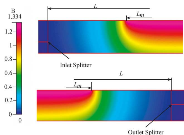
Fig. 3. The fringing field of the magnitude of \mathbf{B} at the separation channel inlet and outlet, B_0 = 1.334 T. Here, variation of the fringing field around the circumference of the annular channel is ignored.
